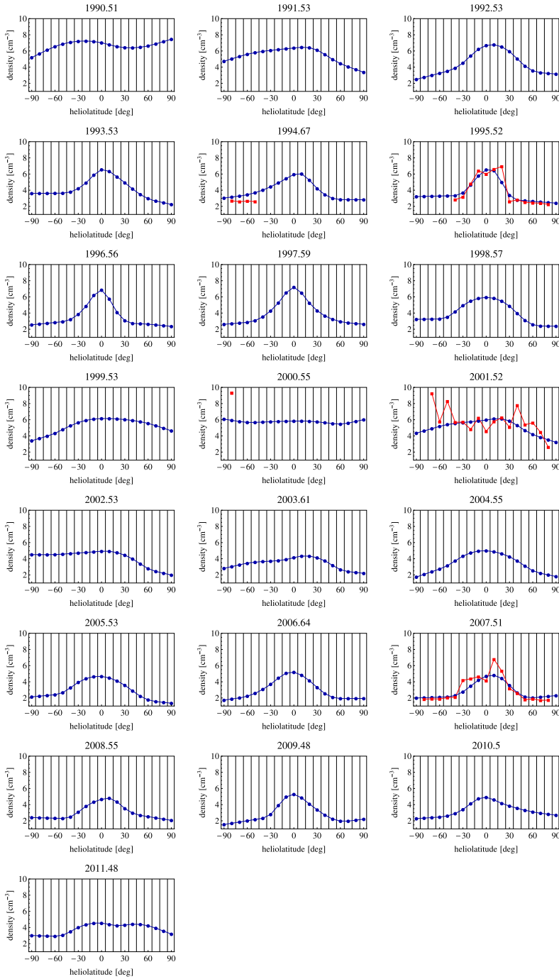
Figure 19 Heliolatitude yearly profiles of solar wind density obtained from the density–speed correlation discussed in the text adopted to the smooth speed profiles obtained in the previous subsection. The red dots and lines show the corresponding parts of the Ulysses fast scan profiles, as in Figure 14. The average times for the profiles are indicated in the panel headers.
